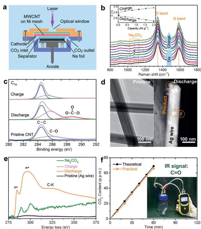
Figure 2. Reaction confirmation of Na-CO 2 batteries, 4\text{Na} + 3\text{CO}_2 \rightleftharpoons 2\text{Na}_2\text{CO}_3 + \text{C} . a) Design of in situ Raman battery. b) In situ Raman spectrum and corresponding discharge/charge profiles with 11 selective points. Rate: 1 A g -1 . c) XPS. d) TEM images of pristine and discharged Ag wire. e) EELS of Ag wire cathode at different states. f) Online CO 2 -evolution test.
