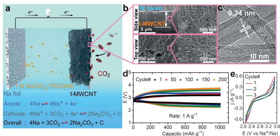
Figure 1. The structure and rechargeability of room-temperature Na-CO 2 batteries. a) Structure of Na-CO 2 batteries with metal Na foil anode, ether-based electrolyte, and t-MWCNT cathode. b) SEM images of cathode from top and side views. c) HRTEM image of t-MWCNT. d) Discharge and charge profiles of Na-CO 2 batteries at 1 A g -1 . e) CV curves of Na-CO 2 batteries with scan rate of 0.1 mV s -1 .
